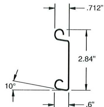
FLAT SLAT 24, 22, 20 OR 18 GA.
