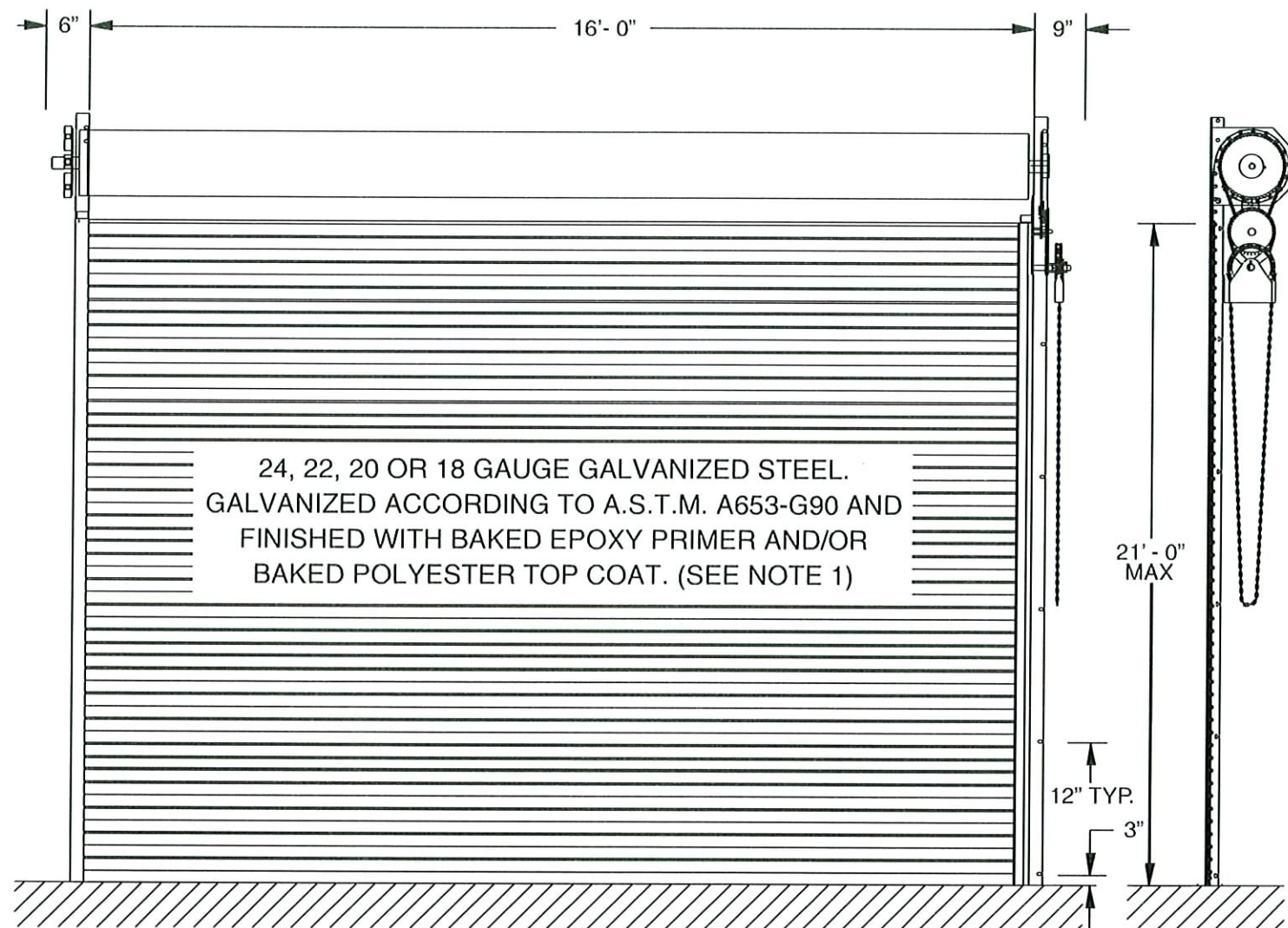
INTERIOR ELEVATION
